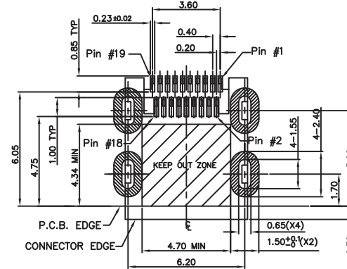
RECOMMENDED PCB LAYOUT TOP VIEW TOLERANCE: ±0.05mm PCB THICKNESS: 0.80±0.05mm
