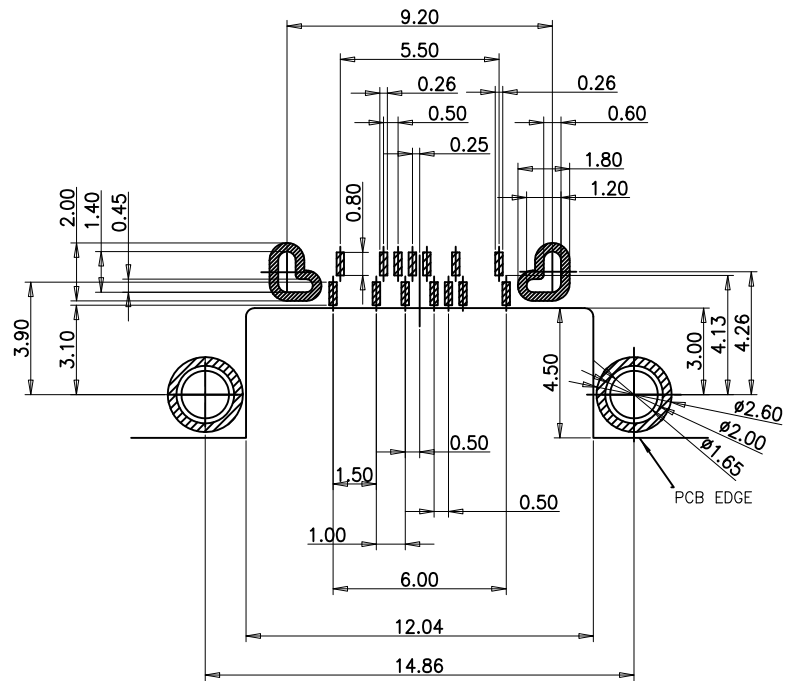
RECOMMENDED PCB PAD LAYOUT TOLERANCE:0.05mm
