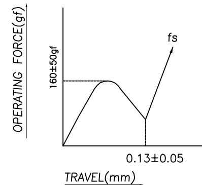
OPERATING FORCE(PUSH)-TRAVEL CHART
